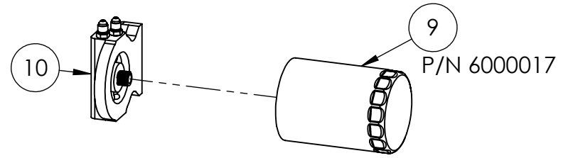
90409100 Bypass Oil Filtration Kit (10 Micron Filtration)
