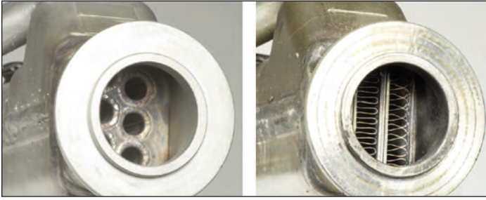
above: Our upgraded EGR Cooler left, Ford Stock Part at right
