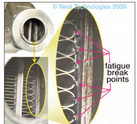
Ford Stock EGR Cooler, core shown
