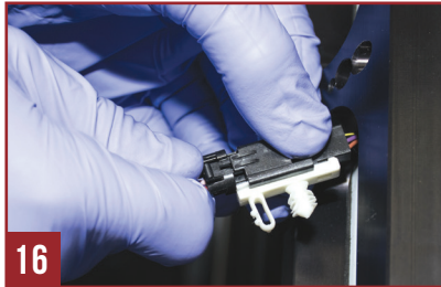
Fig. 16 Re-connect the light housing in the reverse manner as removal. With the power harness attached, route back through the opening and with the clips aligned with the small openings push up to attach backing plate.
