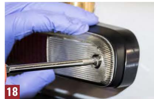
Fig. 16 Route passenger side cab light bulb behind the support bracket and back through the antenna adapter opening. Fig. 17-18 Attach the bulbs to the light housing starting with the passenger side, then middle brake light bulb and finally the driver side. NOTE: The power connectors WILL NOT be re-attached to the anchor point on the light housing. Route the harness and back of the light housing to avoid interference with the antenna cable as it is positioned back in place. Fig. 19 Re-install the light housing utilizing the provided hardware. With the 3rd Brake Light Antenna Adapter installed, attach desired compatible antenna with NMO standard threaded antenna connector and fasten the PL-259 male UHF connector to preferred 2-way radio.
