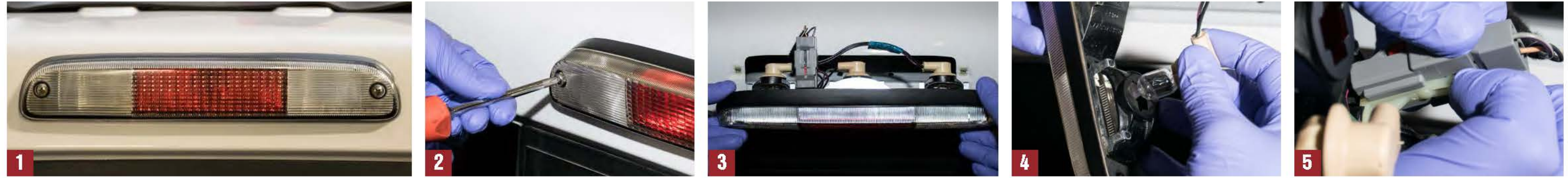
Fig. 2-3 Using a phillips screwdriver, remove the two (2) screws holding the light housing in place and pull away from the cab. Fig. 4-5 Disconnect the light housing by rotating the bulbs counter-clockwise, then pull straight out to remove from the light housing. Next, release the entire harness from anchor point on the housing by pulling back on the retaining clip below the power connectors, then slide away from the housing. NOTE: The power connectors remain connected to each other. Place the removed light housing in a safe location to be re-installed later.
